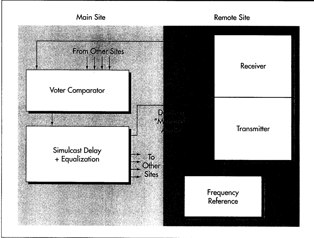
Figure 2: Conventional simulcast system
